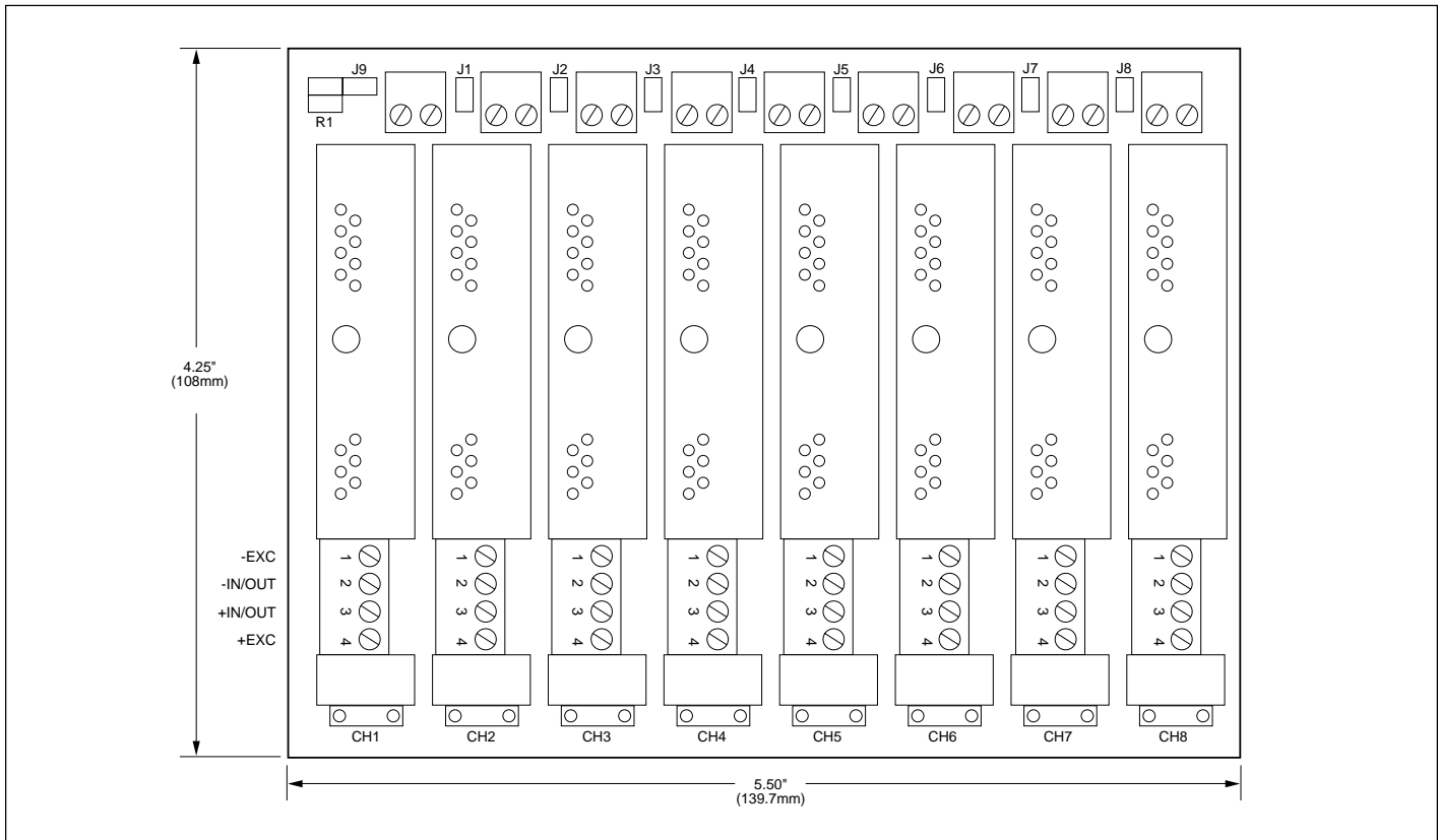
FIGURE 16. SCMPB07 Analog I/O Backpanel.
