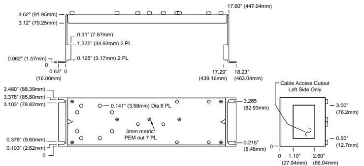
FIGURE 21. SCMXRK-002 Analog Rack Dimensions.
