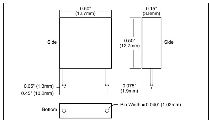
FIGURE 24. SCMXR1 Physical Dimensions.
