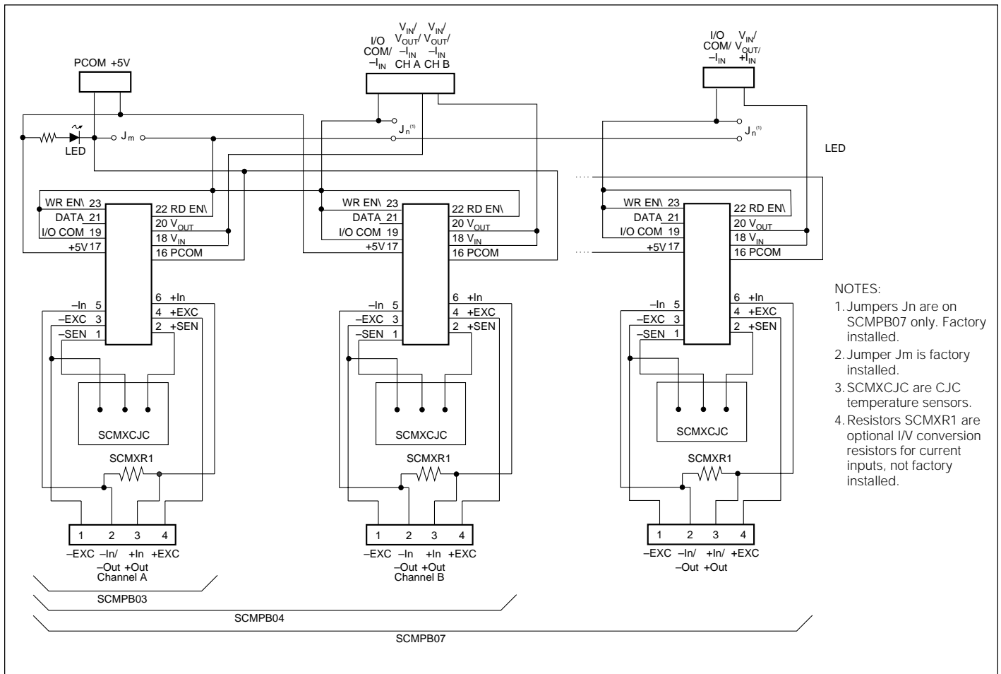
FIGURE 11. SCMPB03/SCMPB04/SCMPB07 Schematic.
