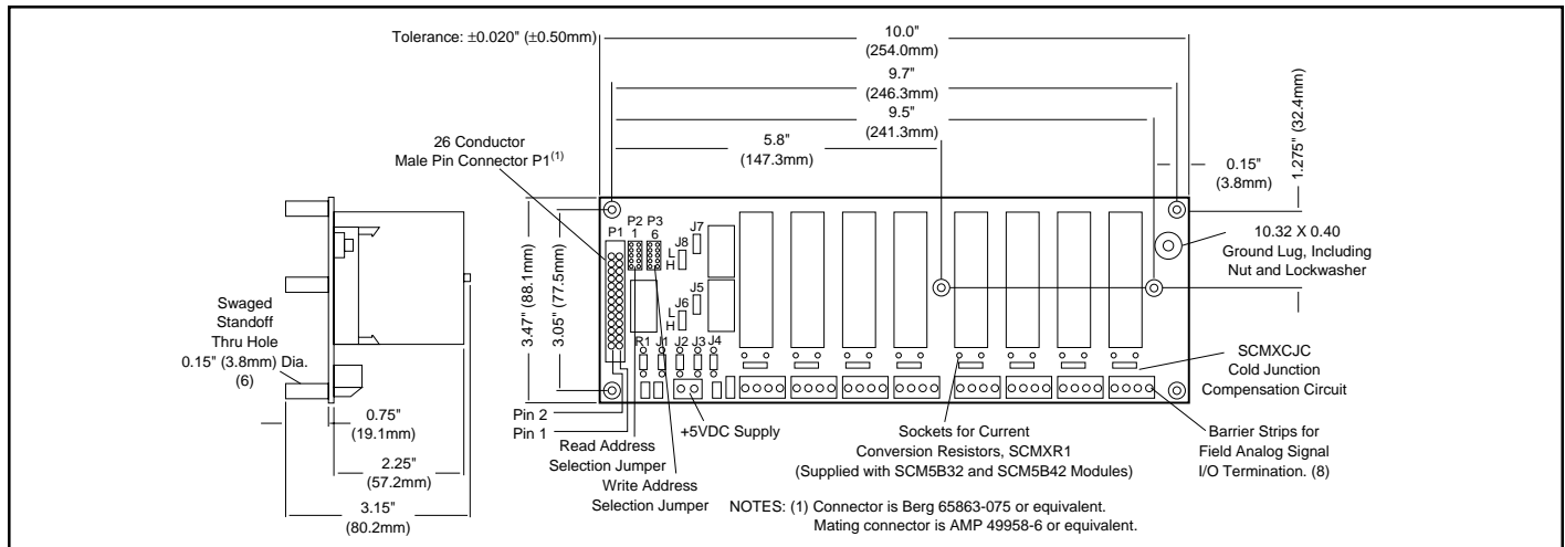
FIGURE 14. SCMPB06 Analog I/O Backpanel.
