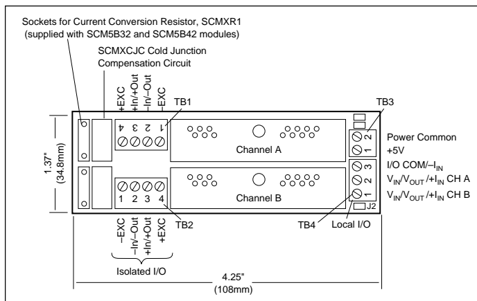
FIGURE 10. SCMPB04 Analog I/O Backpanel.
