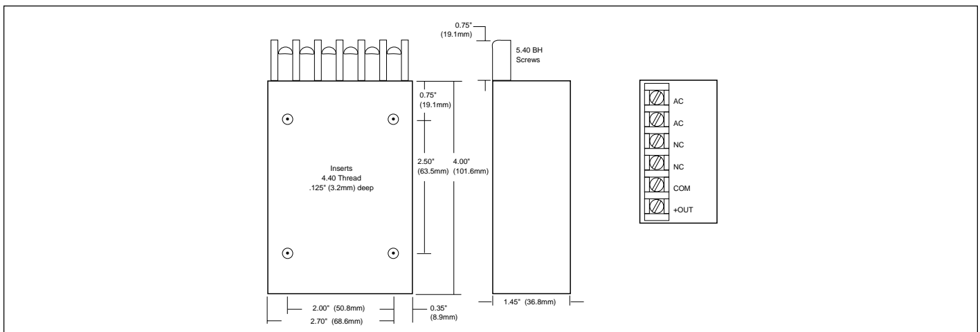
FIGURE 26. SCMXPRT-001/E-001 Physical Dimensions.
