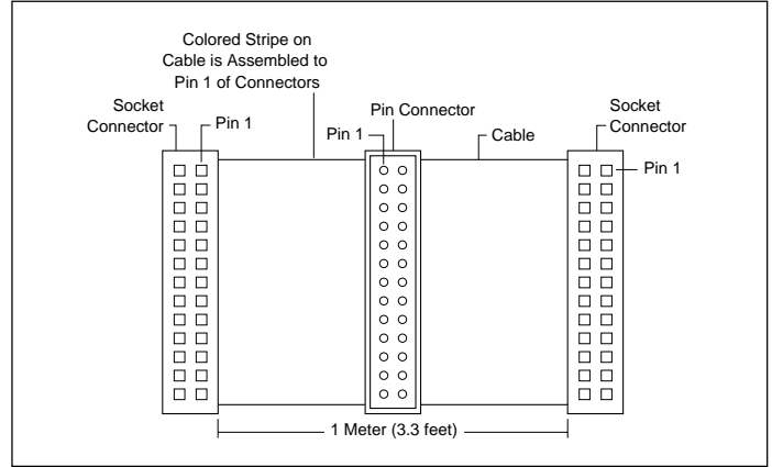
FIGURE 20. SCMXCA005 Daisy-Chain Cable.
