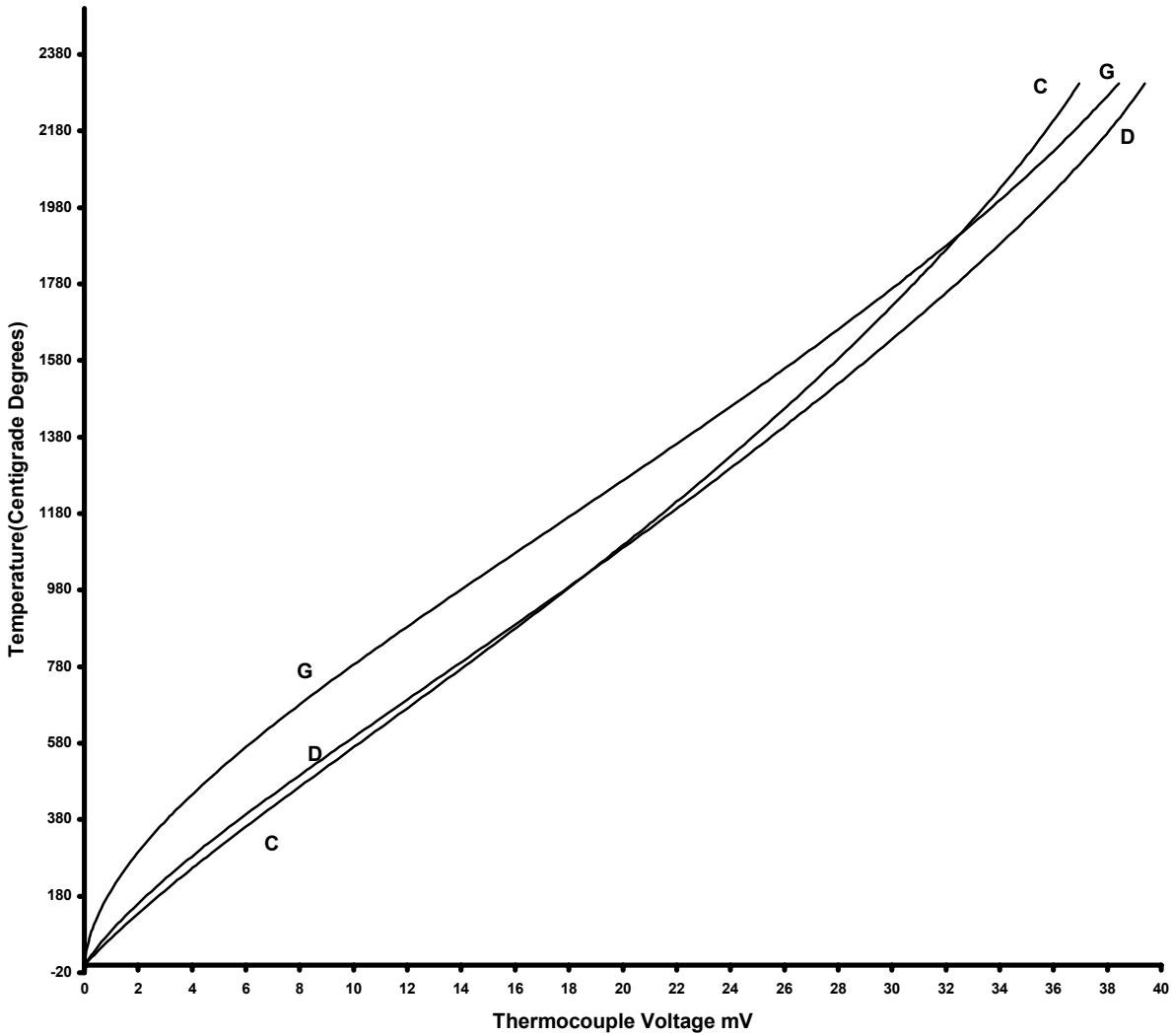
Figure 4 Voltage-Temperature Characteristics of G, D, C Type Thermocouples
